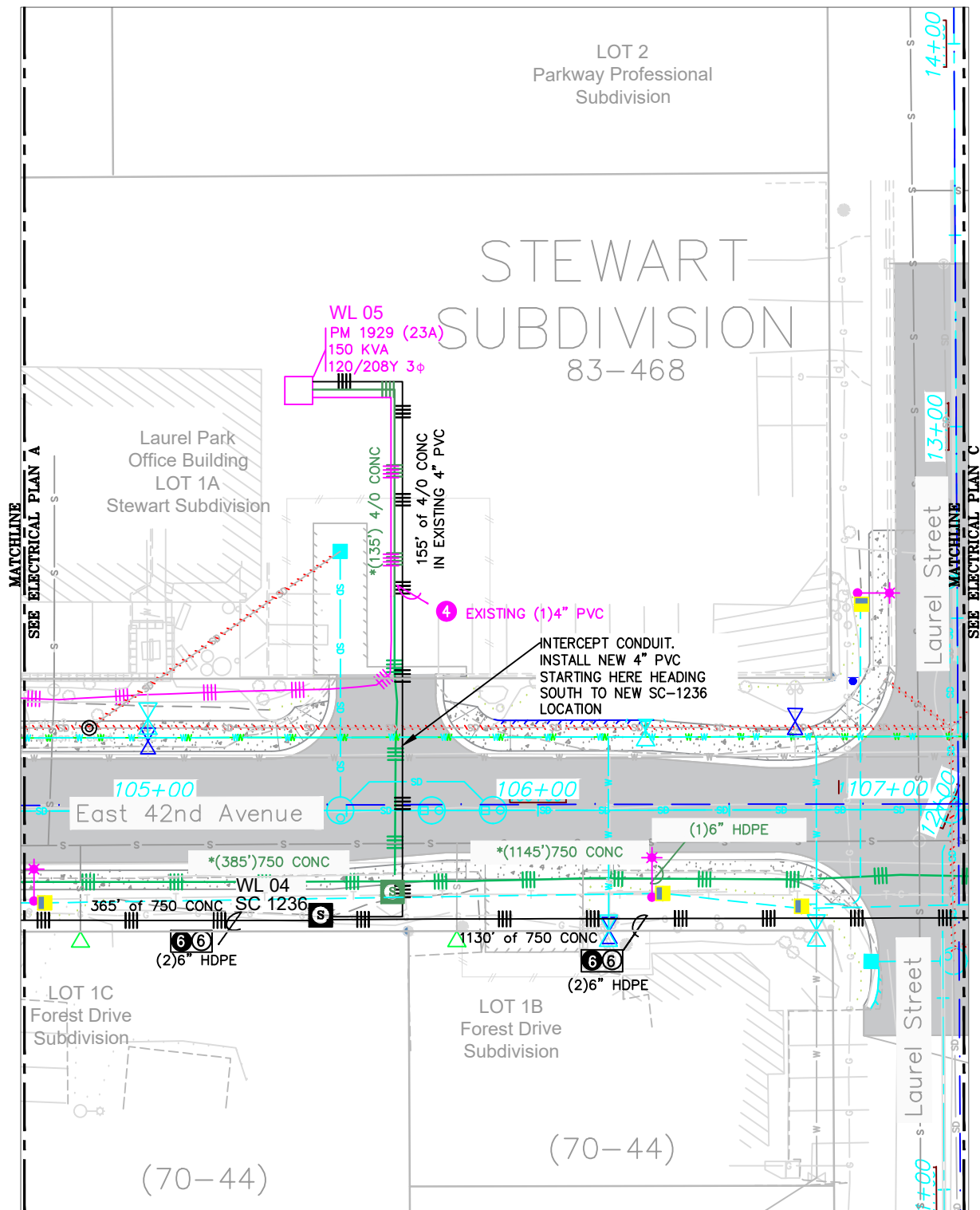
ELECTRICAL PLAN B SCALE = 1:40
