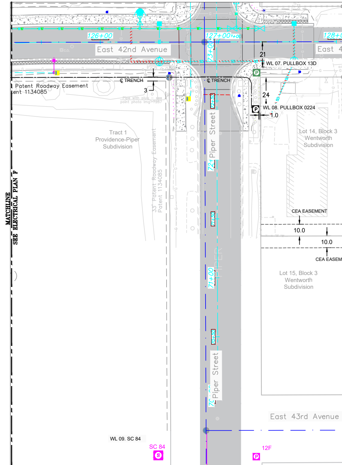
RIGHT-OF-WAY PLAN G SCALE = 1:50
